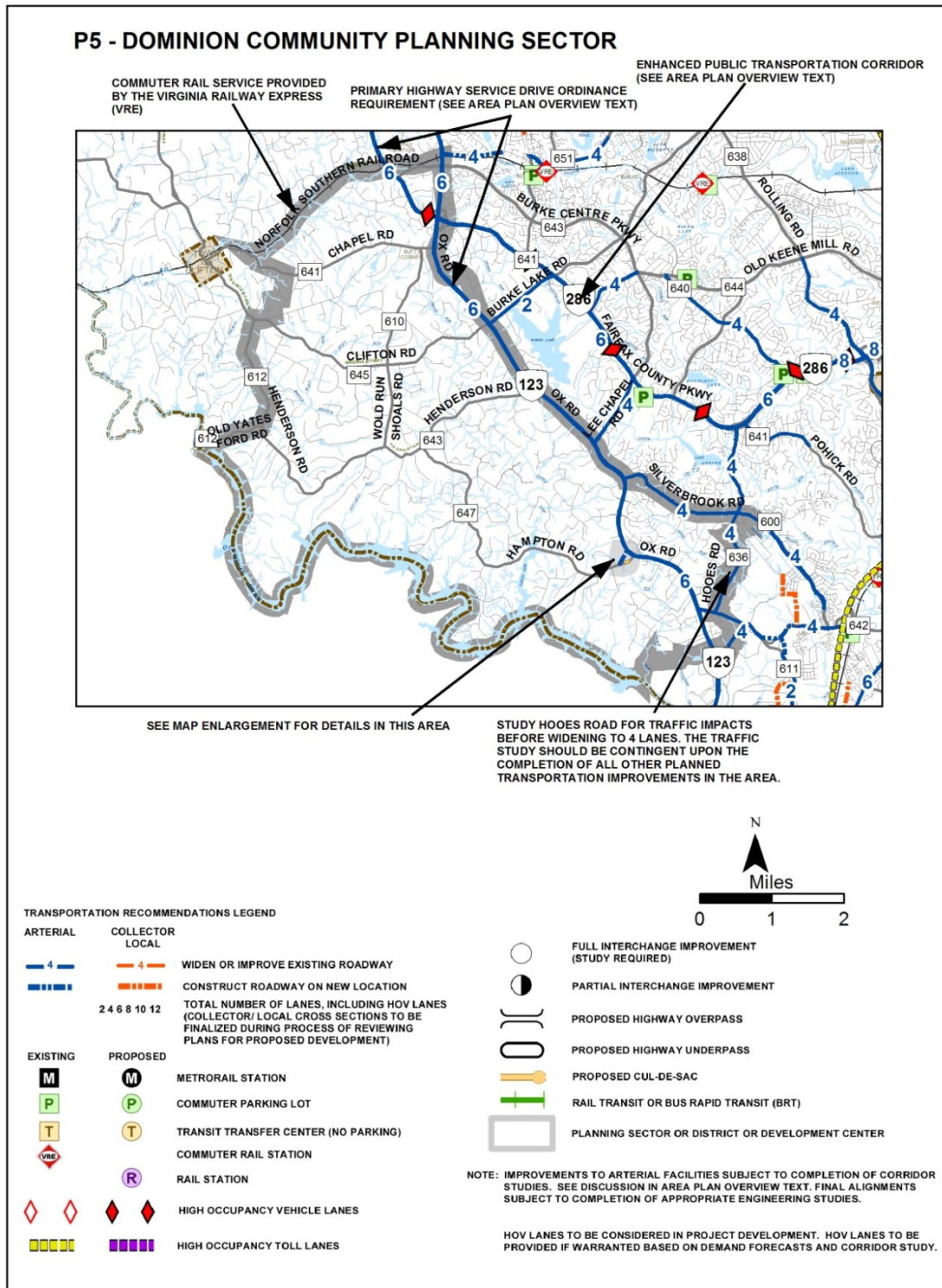
INTERSECTION REALIGNMENT RECOMMENDATIONS P5 COMMUNITY PLANNING SECTOR
